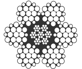
6x19 WARRINGTON 6(1+6(6+6))
