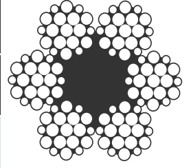
6*19 WARRINGTON 6(1+6+(6+6))
